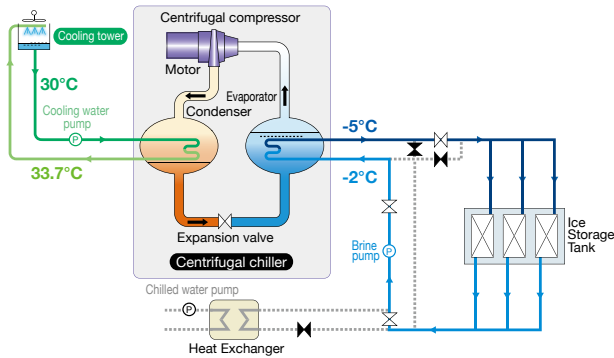
System Flow [Ice Charge Mode (Night)]
