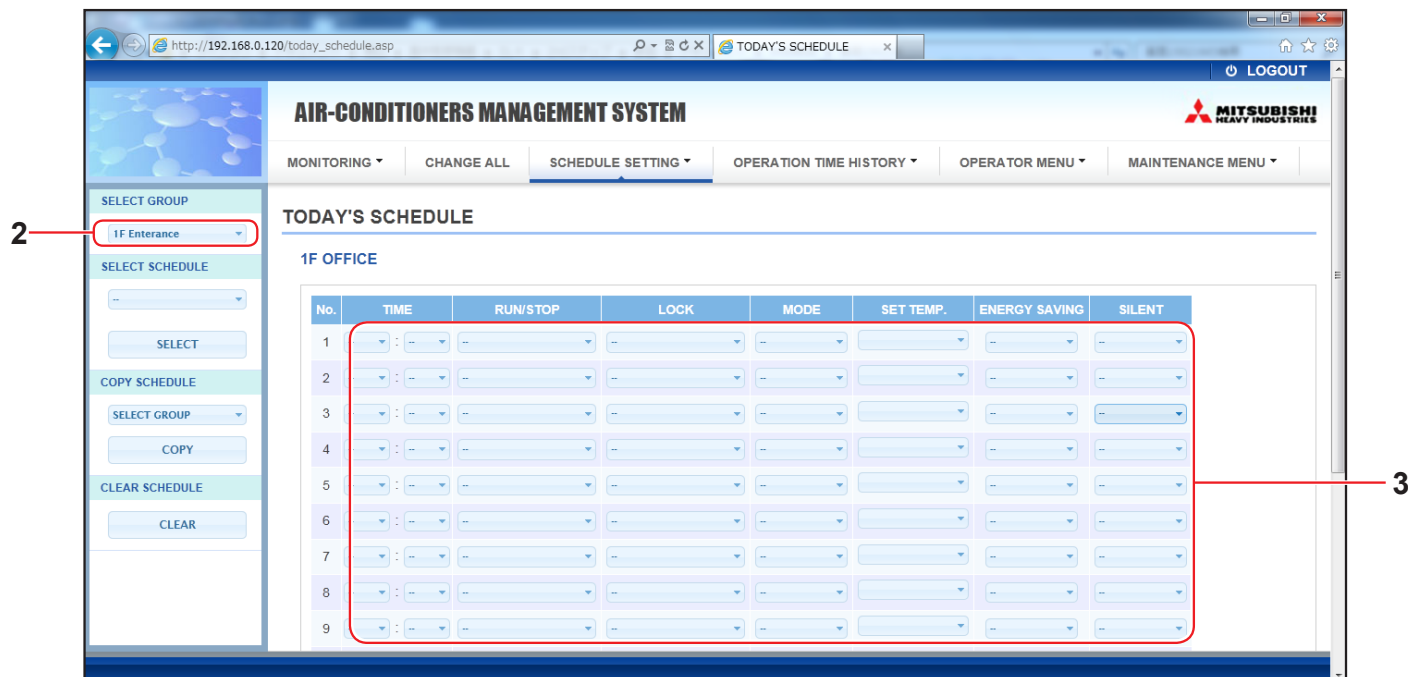
TODAY'S SCHEDULE-scherm
