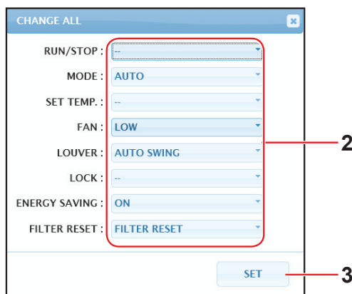
CHANGE ALL-scherm
