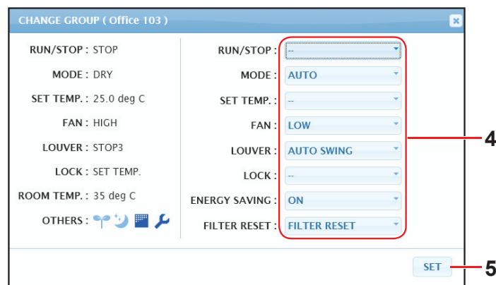
CHANGE GROUP-scherm
