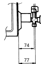
A部詳細 (HCA15R)
