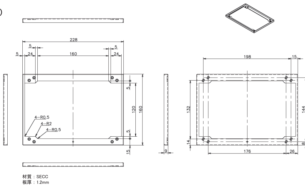
(c) 取付金具(裏)
